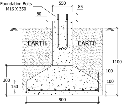
Pole Foundation (Upto 5 Mtrs.)
