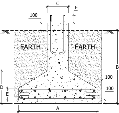
Pole Foundation (6-9 Mtrs.)
